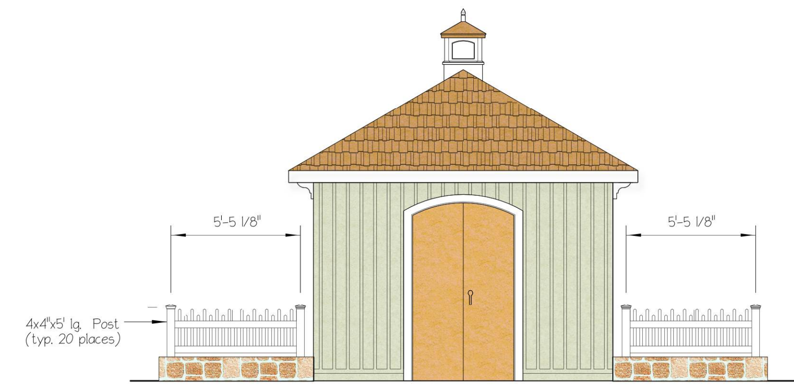
POTAGER GARDEN FENCE DETAIL (Shed End Elevation) Scale: 1/4" = 1'-0"
